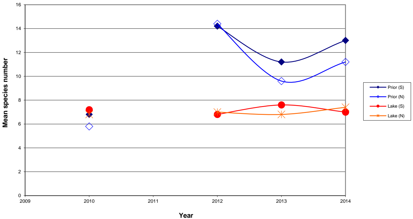
Figure 10.11 Changes in species-richness at Priors Ham and Lake Meadow 2010–14. Lake Meadow (S) and (N) are two blocks of quadrats in the control field.
